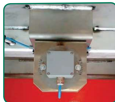
Body-mounted inclinometer (unique to 1300 BulkWeigh)
